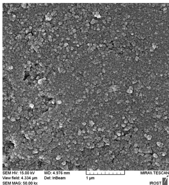
Fig. 2 — SEM image of Fe 3 O 4 nanoparticles.
