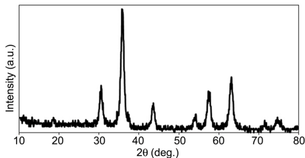
Fig. 1 — XRD pattern of Fe 3 O 4 nanoparticles.
