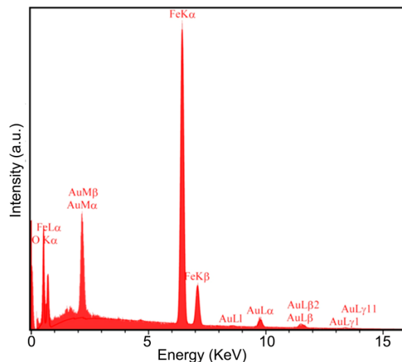
Fig. 3 — EDS analysis of Fe 3 O 4 nanoparticles.
