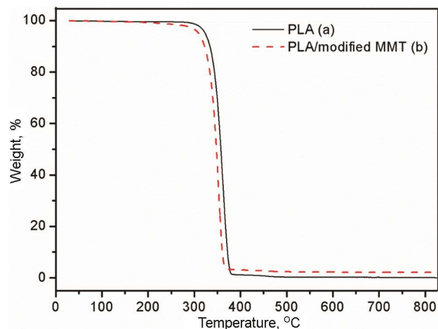
Fig. 3 — TGA of (a) PLA and (b) PLA/modified MMT nanocomposite
