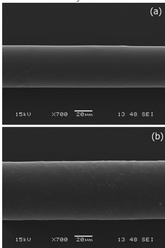
Fig. 2 — SEM micrographs of (a) PLA and (b) PLA/modified MMT nanocomposite fibre
