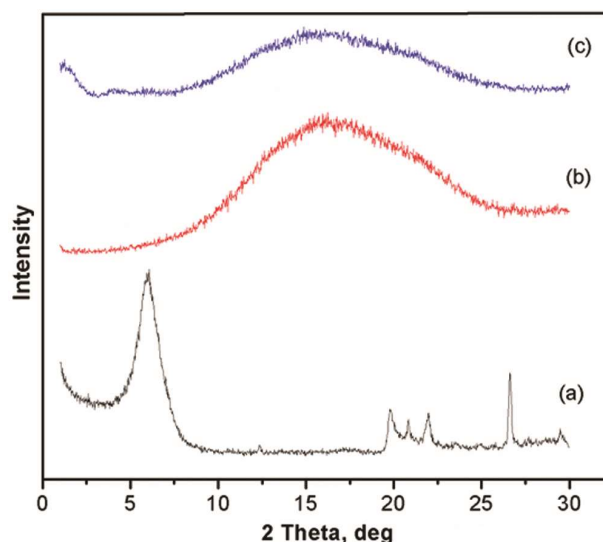
Fig. 1 — XRD patterns of (a) MMT, (b) PLA, and (c) PLA/modified MMT nanocomposite
