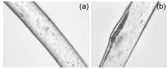
Fig. 2 — Microscopic view of PES R fibres at a magnification of x1000 [(a) impurities and (b) cracks]
