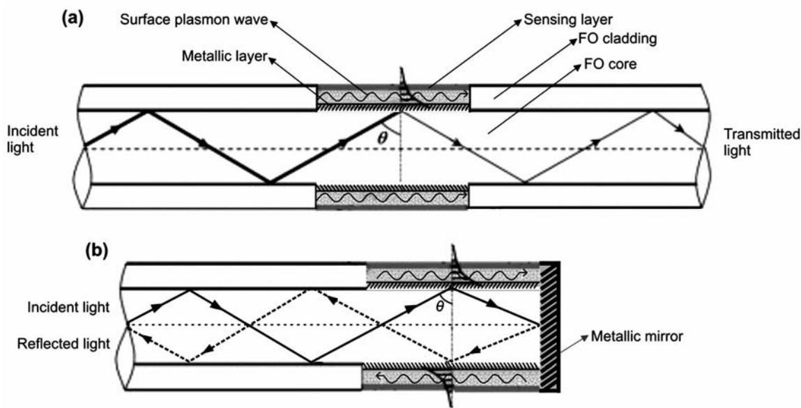
Fig. 4 — Illustration of a typical FO-SPR configuration for the excitation of surface plasmon at metal-dielectric interface at core-cladding junction of optical fiber (a) intermediate FO zone as sensing area and (b) tip as sensing area
