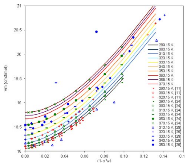
Fig. 5—Experimental and calculated molar volume of aqueous solutions of \text{CaCl}_2
