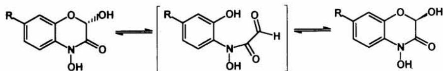
Scheme I – Oxo-cyclo tautomerism of natural hemiacetalic hydroxamic acids
