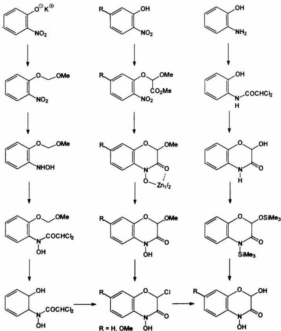
Scheme II—Literature syntheses leading to the 2,4-dihydroxy-2H-1,4-benzoxazin-3(4H)-one skeleton
