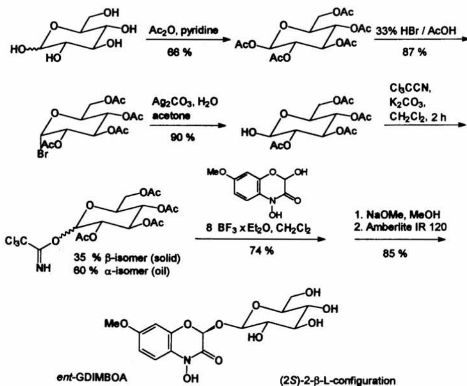
Scheme XIII—Stereoselective synthesis of ent -GDIMBOA
