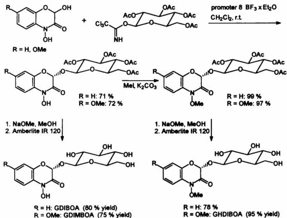
Scheme XII—A synthesis of GDIMBOA and GDIBOA with double (2 R )-2- \beta -diastereoselectivity
