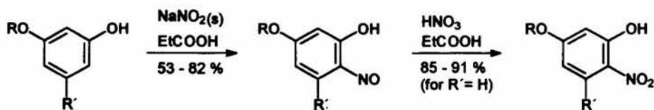
Scheme VII—Regioselective nitrosation of resorcinol monoethers and oxidation to 2-nitrophenols
