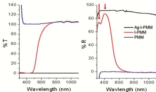
Fig. 4 – Change of % T and % R with wavelength of PMM, iodine-PMM and silver-iodine-PMM
