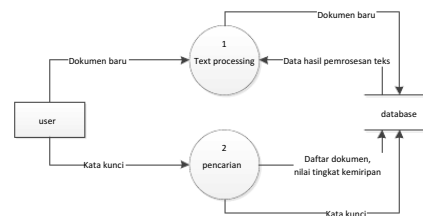
Gambar 5. DFD Level 1 Sistem information retrieval
