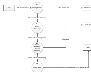
Gambar 6. DFD Level 1.1 Parsing kalimat
