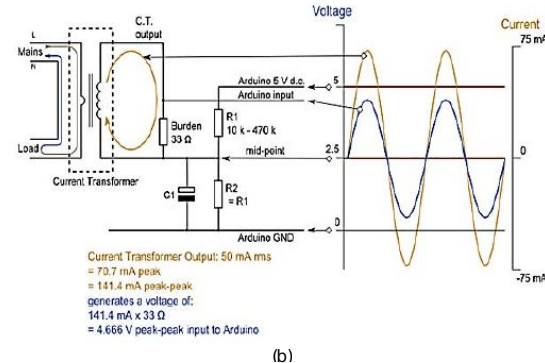
Fig. 4 Current transformer diagram, (a) Primary and secondary side schemes of current transformer [14], (b) Signal conditioning circuit to microcontroller ADC [15]
