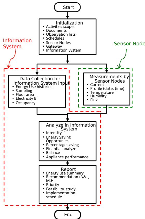
Fig. 10 Flow Diagram of Electronic Energy Audit Process
