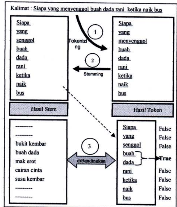
Gambar 8. Proses Phrase Porn Filtering
