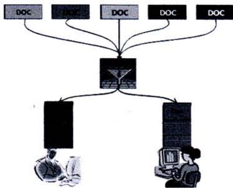
Gambar 1. Information Filtering
