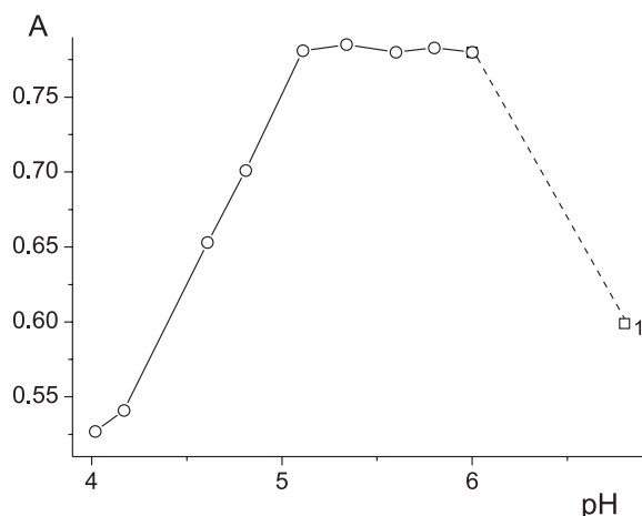
Fig. 1. The dependence of absorption of the ellagitannin complex of Altabor with ions of iron (II) on pH. The retention time is 120 min. \lambda = 550 nm. l = 10 mm. The reference solution is water.
