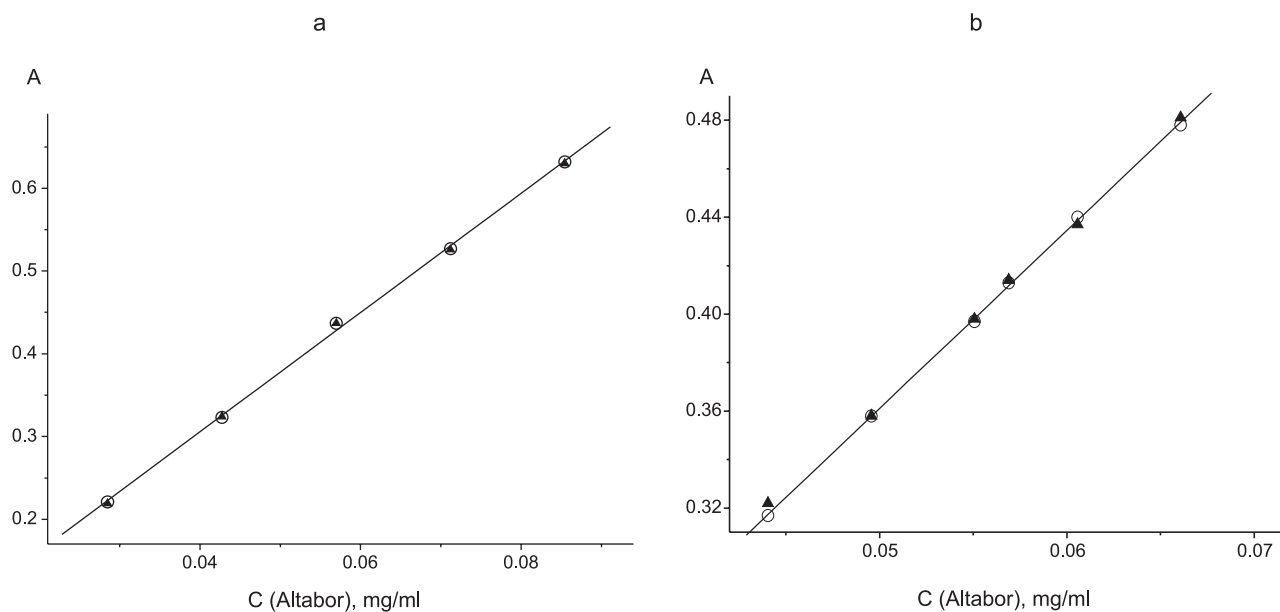
Fig. 3. Absorption of the complex of iron (II) with ellagitannins of Altabor of batches 30905 (a) and 51005 (b) in the medium of acetate buffer with pH 5.30 at 550 nm. Compensation solution – water.
