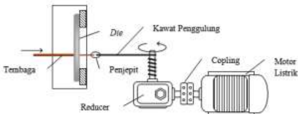
Gambar 1. Mekanisme alat wire drawing
