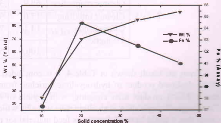
Fig. 2: Effect of solid concentration on flotation of iron ore.
