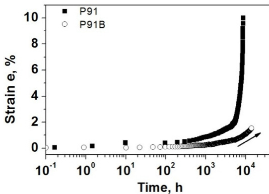
Figure 6: Creep curve of P91 and P91B tested at 600°C and 100MPa
