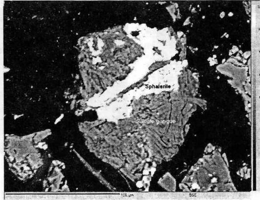
Fig. 4: (Zinc Tails) Back Scattered Electron (BSE) Image Showing the Distribution of Sphalerite (White) (I) Along the Cleavage/Fracture Planes of the Silicate Gangue Minerals (Gray) and (II) Also as Fine to Extremely Fine Inclusions in the Silicate Gangue
