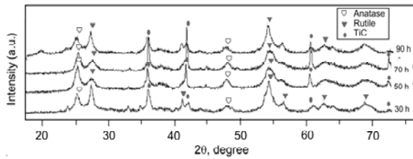
Figure 5. XRD patterns for \text{TiO}_2 -graphite powders milled for various durations (30 h, 50 h, 70 h, and 90 h) and heat treated at 1300\text{ }^\circ\text{C} for 2 hours
