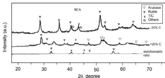
Figure 2. XRD patterns for as milled TiO 2 -C mixed powders with various graphite contents and milled for a constant milling time of 90 hours
