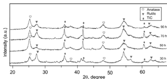
Figure 4. XRD patterns for TiO 2 -graphite powders milled for various durations (30 h, 50 h, 70 h, and 90 h) and heat treated at 1300 °C for 1 hour
