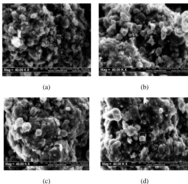
Figure 3. SEM images of as milled TiO 2 -graphite mixtures after milling for (a) 30 h (b) 50 h (c) 70 h and (d) 90 h
