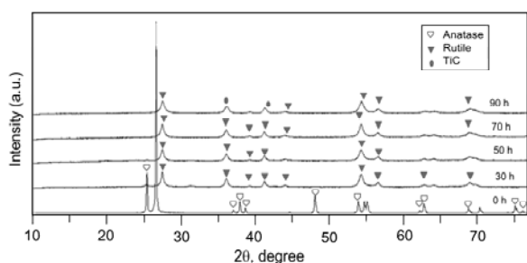
Figure 1. XRD patterns for as milled TiO 2 -C mixed powders with stoichiometric carbon milled for various durations
