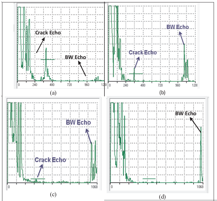
Fig. 5: Ultrasonic signals at 1280 mm from the work side with crack depths of (a) 5.965 mm, (b) 1.465mm, (c) 0.43 mm and (d) no crack
