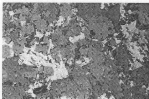
Fig.1 : Chalcopyrite occurring at inter-granular grain boundaries of the silicates.
