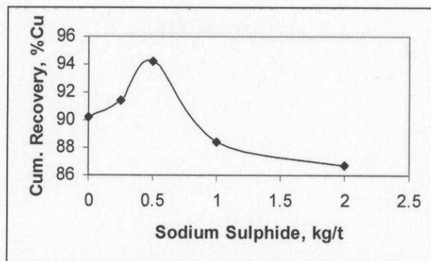
Fig. 7 : Effect of sodium sulphide on copper recovery.
