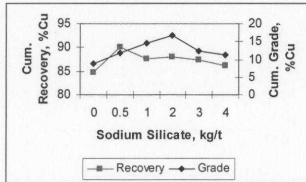
Fig. 6 : Effects of sodium silicate of floatability of copper minerals.
