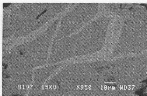
Fig. 2: Back-scattered image of bornite with covellite veins.
