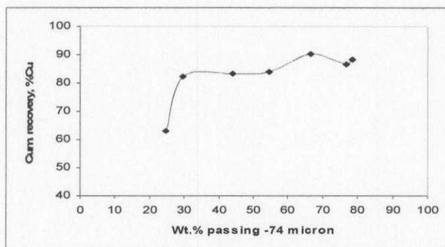
Fig. 3 : Effect of particle size on copper recovery.
