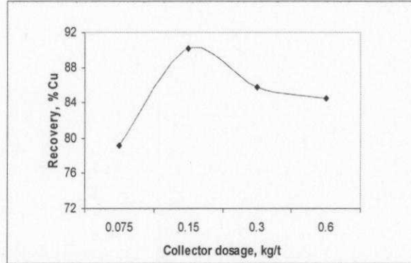
Fig. 4 : Flotation results with varying dosage of collector.
