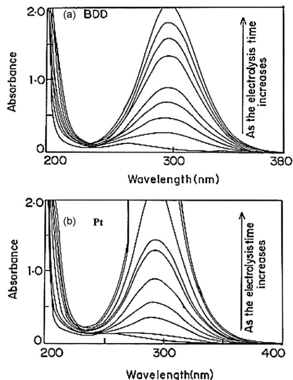
Fig. 6. UV-vis spectra showing \text{OCl}^- during electrolysis (ketoprofen: 5 \mu\text{M} , applied current density: 8.8 \text{ mA cm}^{-2} , \text{NaCl} : 0.1 \text{ M} , initial pH: 6.00, T : 25^\circ\text{C} ).
