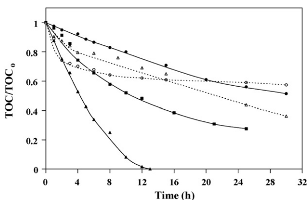
Fig. 8. Effect of supporting electrolyte on TOC removal (electrolyte concentration: 0.1 M, ketoprofen: 5 \mu\text{M} , initial pH: 6.00, T: 25^\circ\text{C} , applied current density: 8.8 \text{ mA cm}^{-2} , (●) BDD–NaCl, (▲) BDD– \text{Na}_2\text{SO}_4 , (■) BDD– \text{NaNO}_3 , (○) Pt–NaCl, (△) Pt– \text{Na}_2\text{SO}_4 ).
