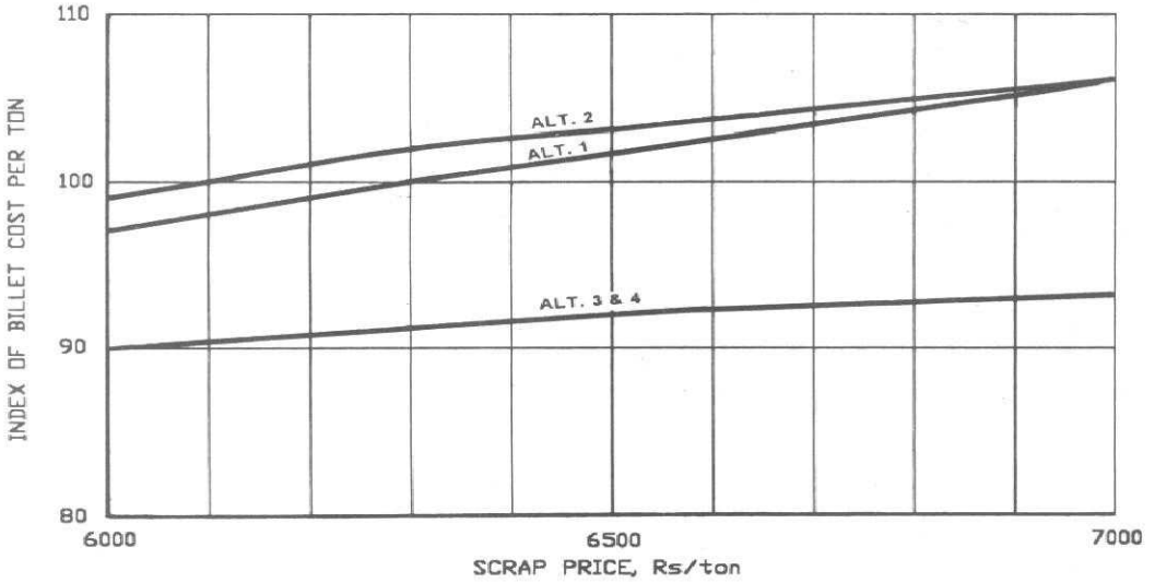
Fig.3 : Billet cost Vs scrap price
