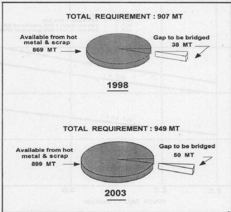
Fig.2 : Future world metallics situation
