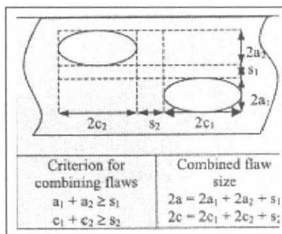
Fig. 7 : Suggested rules for combining flaws in API 579
