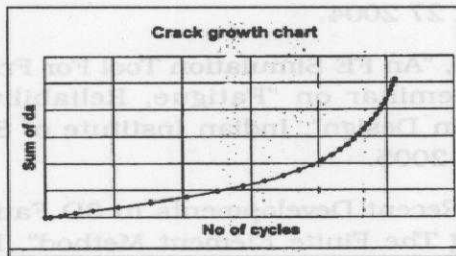
Fig. 9 : Crack growth - cyclic bending of a pipe
