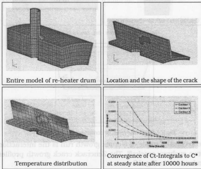
Fig. 5 : Reheater drum - an example of creep
