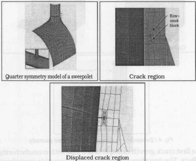
Fig. 3 : Sweepolet - an example of a parametric study
