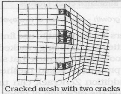
Fig. 8 : Multiple flaws - a nozzle
