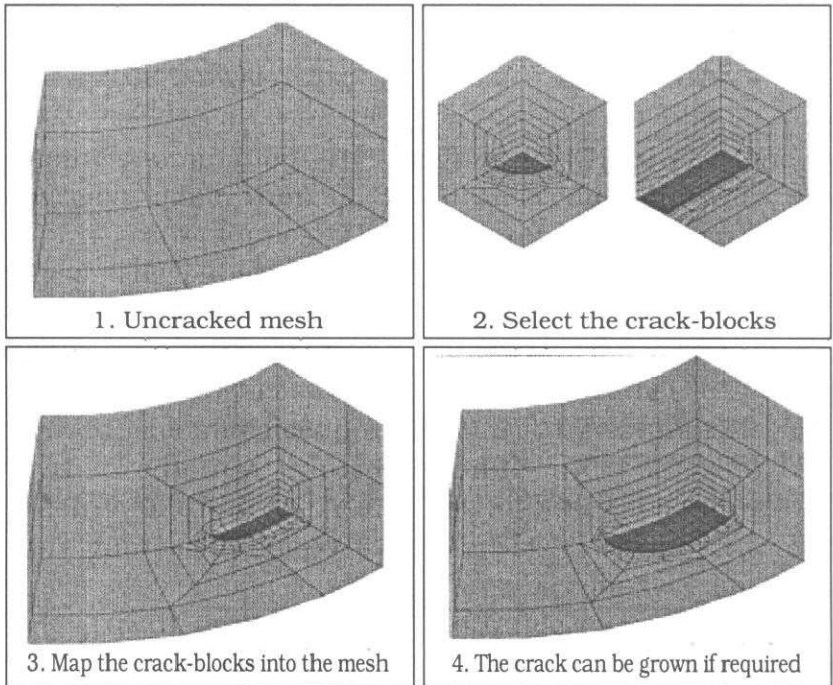
Fig. 1 : Inserting a crack into a mesh using Zencrack
