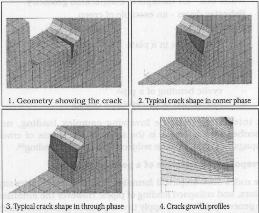
Fig. 2 : Demonstration of crack growth using ZenCrack
