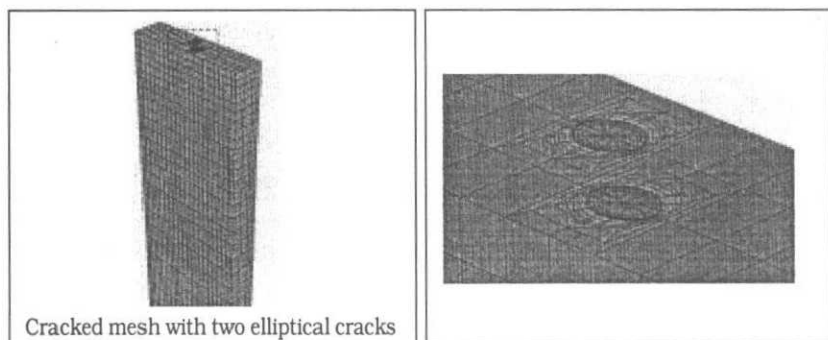
Fig. 6 : Multiple flaws - two cracks in a plate
