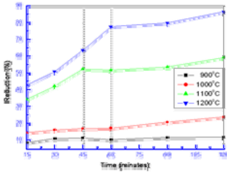
Fig. 11: Effect of temperature on the reducibility of multi-metallic magnetite ore (- 5 mm + 6 mesh) using low ash coke as reductant in solid-solid system.
