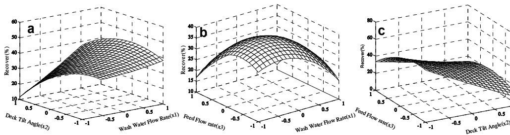
Fig. 4: Response surface plots showing the effects on recovery (%) of Cr_2O_3 in the concentrate fraction: (a) Between wash water flow rate ( x_1 ) and deck tilt angle ( x_2 ), (b) Between wash water flow rate ( x_1 ) and feed flow rate ( x_3 ), (c) Between deck tilt angle ( x_2 ) and feed flow rate ( x_3 ).
