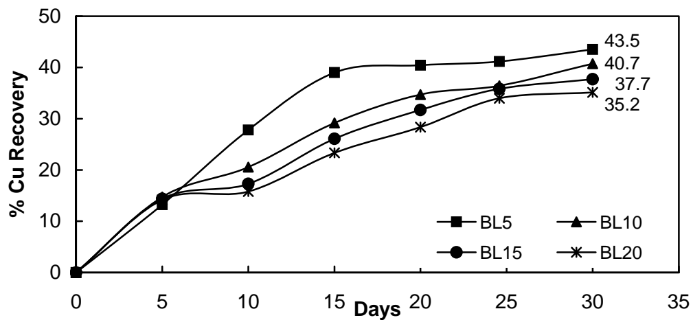
Fig. 3:- Effect of pulp density on bio-leaching of copper by bacterial consortium with particle size of
