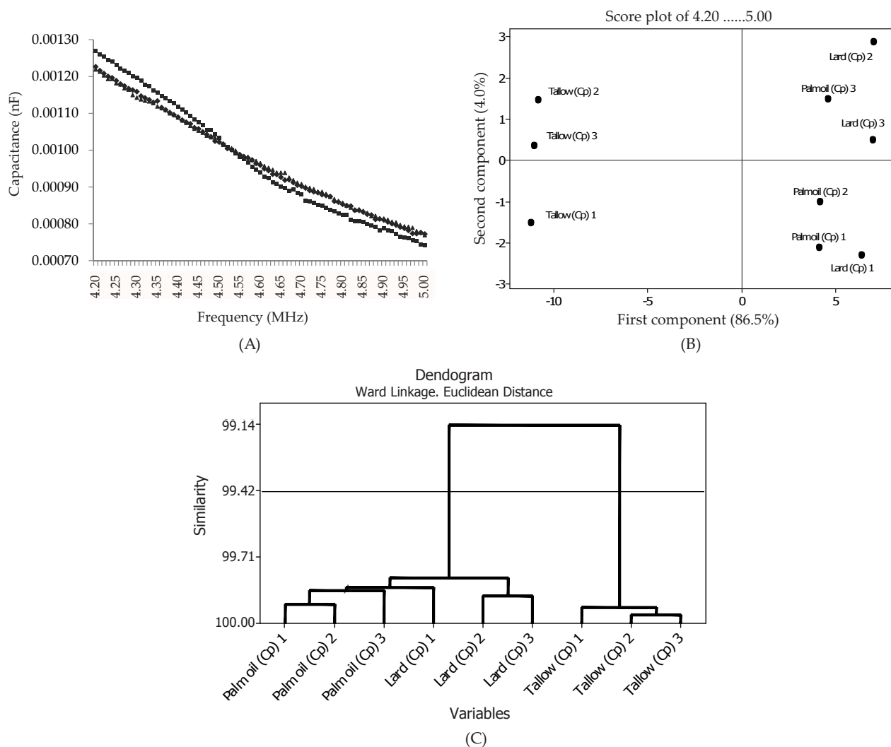
Figure 3. Capacitance of samples (lard: -▲-, tallow: -■-, and palm oil: -◆-). (A) The relations frequency with a capacitance of samples; (B) The score plot for the first two principal components (PC) for capacitance of samples; and (C) Dendrogram illustrating the stages of clustering of the evaluated samples based on capacitance.
