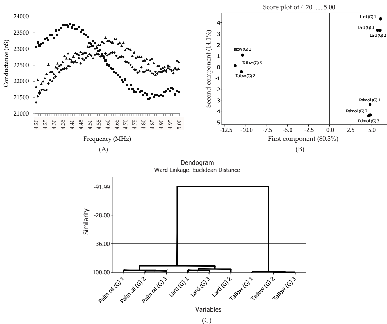
Figure 1. Conductance of samples (lard: -▲-, tallow: -■-, and palm oil: -◆-). (A) The relations frequency with a conductance of samples; (B) The score plot for the first two principal components (PC) for conductance of samples; (C) Dendrogram illustrating the stages of clustering of the evaluated samples based on conductance.
