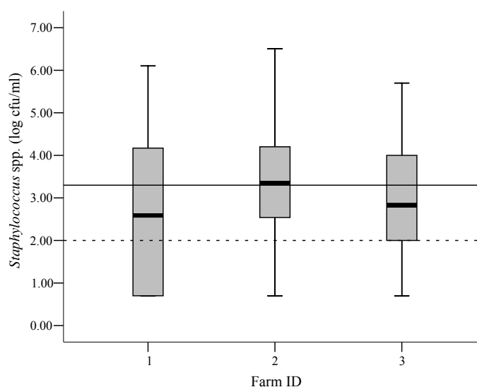
Figure 1. Box and Whisker plots of Staphylococcus spp. counts in three farms compared to the maximum limit of available standards ( — = SNI, ..... = EC Directive and "Milchverordnung").
