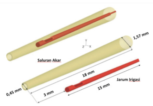
Figure 2. The design of shape and size of root canal test specimen. 17
