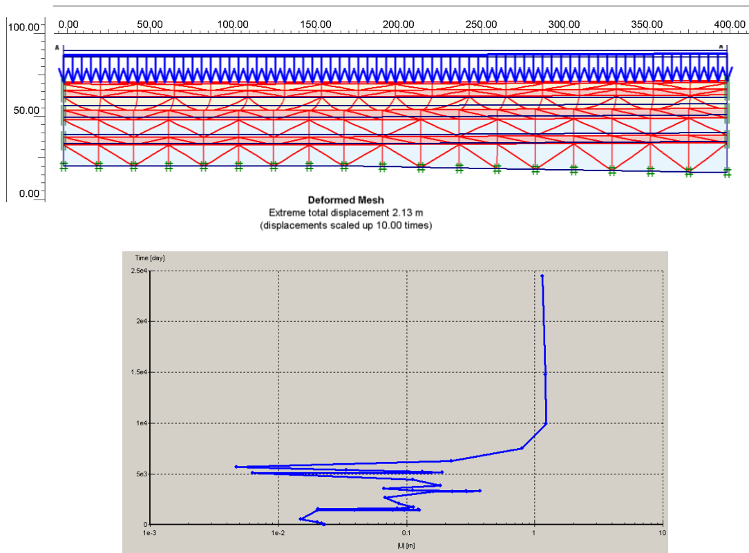
Figure 9. Deformed mesh and displacement (U) versus time plot for section 1 using scenario B The summary result for all sections and comparison with Terzaghi method is shown in Figure 11.
