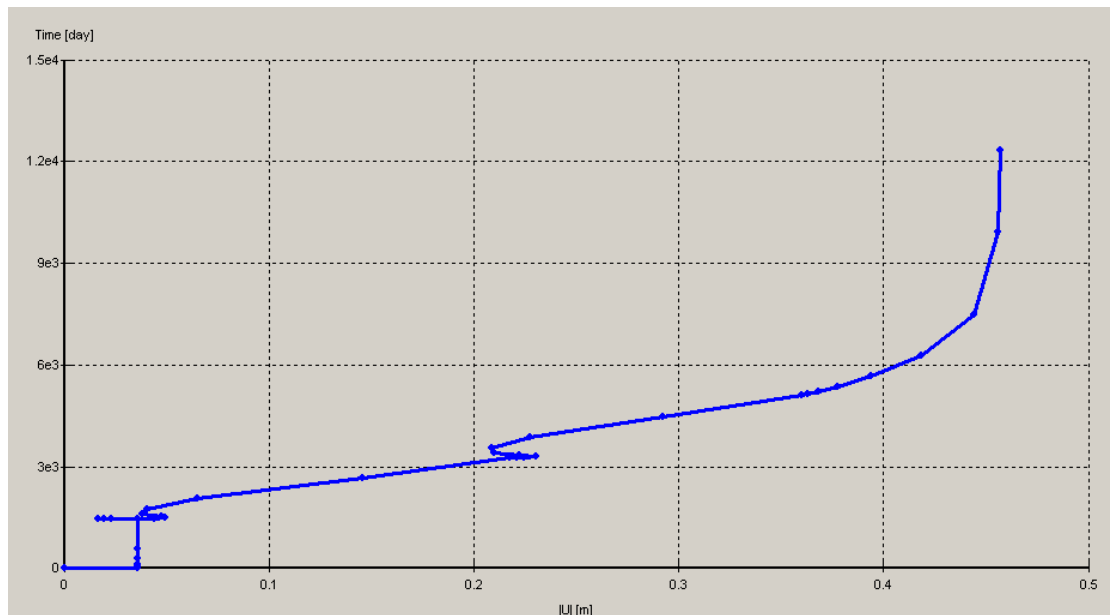
Figure 7. Deformed mesh and displacement (U) versus time plot for section 1 using scenario A
