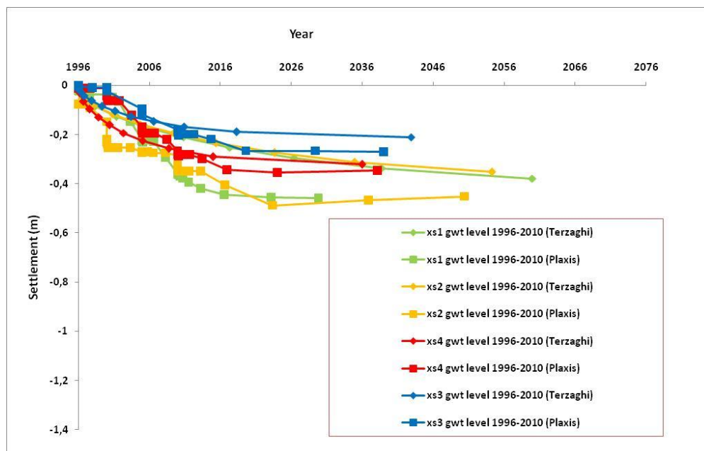
Figure 8. Results of numerical modeling for scenario A
