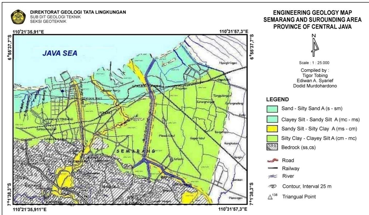
Figure 2. Engineering geological map of Semarang City (Tobing et al., 2001)
