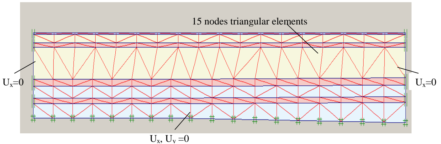
Figure 5. Boundary condition of consolidation modeling
