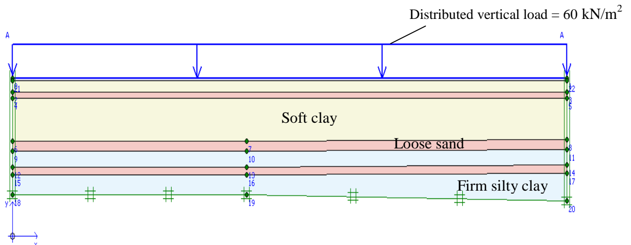
Figure 6. Application of surface load during consolidation modeling
