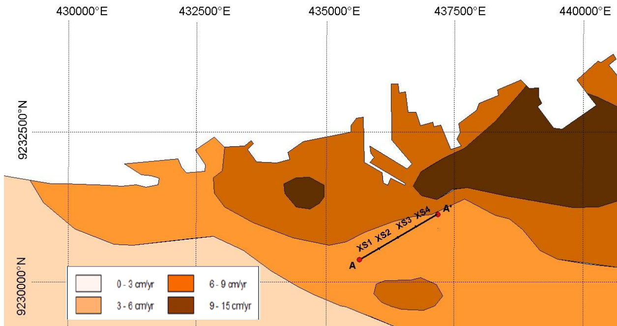
Figure 12. Map of GPS derived zones of subsidence rate in Semarang showing selected A-A' section (modified from Abidin et.al, 2010)
