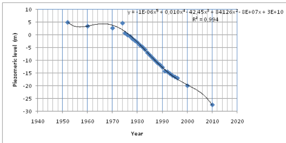
Figure 4. Piezometric levels at Pelabuhan area, Semarang from 1952-2010
