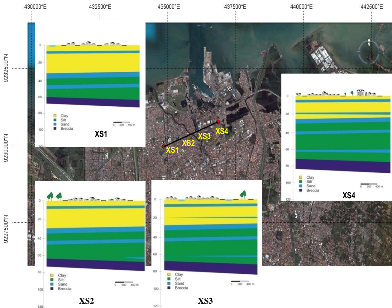
Figure 3. Location of Tanah Mas-Pelabuhan (A-A') and Soil stratification of Tanah Mas-Pelabuhan (A-A') section (modified after Marsudi ,2001).
