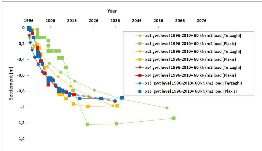
Figure 10. Results of numerical modeling for scenario B
