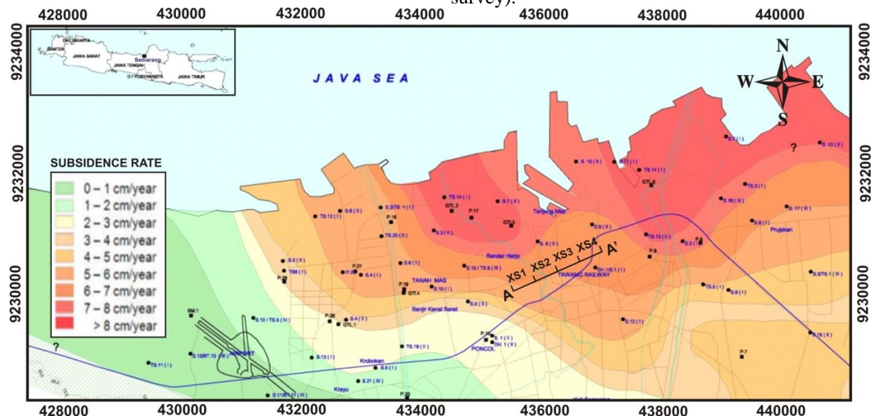
Figure 11. Map of PSI derived zones of subsidence rate in Semarang showing selected A-A’ section (modified from Kuehn et.al, 2009)
