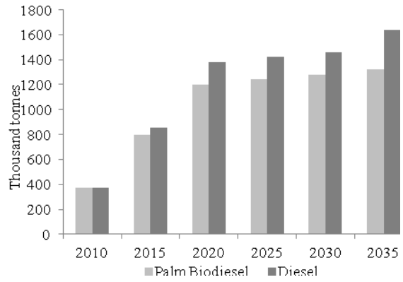
Figure 7. SO 2 emission under the trend and alternative scenario in the Indonesian power generation sector, JAMALI region
