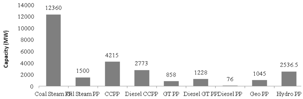
Figure1. Power generation configuration in JAMALI, 2009.
