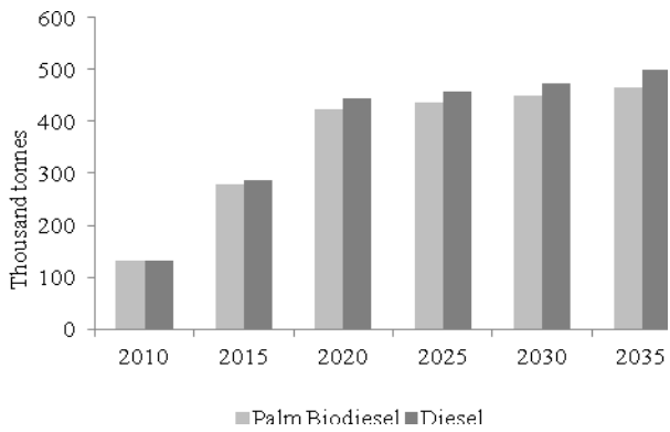
Figure 8. PM 10 emission under the trend and alternative scenario in the Indonesian power generation sector, JAMALI region
