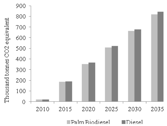
Figure 5. CO emission under the trend and alternative scenario in the Indonesian power generation sector, JAMALI region
