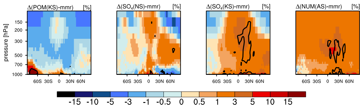
Fig. 13. Ship-emission induced five-year annual zonal mean relative changes in [%] of (from left to right) POM(KS), sulfate(NS and KS) mass mixing ratios and total number mixing ratio in AS in experiment BnoC compared to experiment B derived from \left(\frac{\text{BnoC}-\text{B}}{\text{B}} \cdot 100\right) . Please note the non-linear contour spacing. The black contour lines enclose areas showing statistical significance at the 90 % level.
