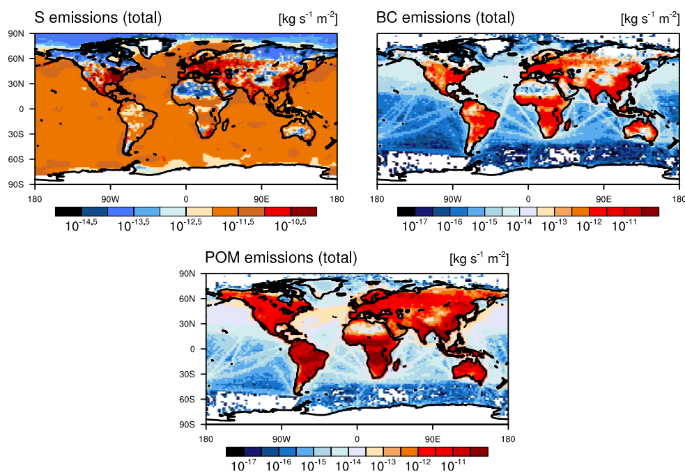
Fig. 1. Total emissions of aerosols and aerosol precursors as used in experiment setup B. Top left: sulphur (comprised of sulphur dioxide ( \text{SO}_2 ), sulfate and DMS); top right: BC; bottom: particulate organic matter (POM). The colour scales denote the \log_{10} of emission fluxes in [\text{kg s}^{-1} \text{m}^{-2}] . Emissions over land correspond to those prescribed in AeroCom (Dentener et al., 2006), anthropogenic emissions over water surfaces to those provided in the QUANTIFY shipping emission inventory (Behrens, 2006).
