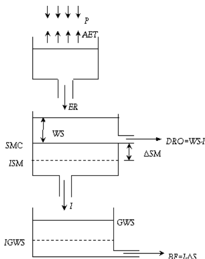
Gambar 1. Model tangki Mock
