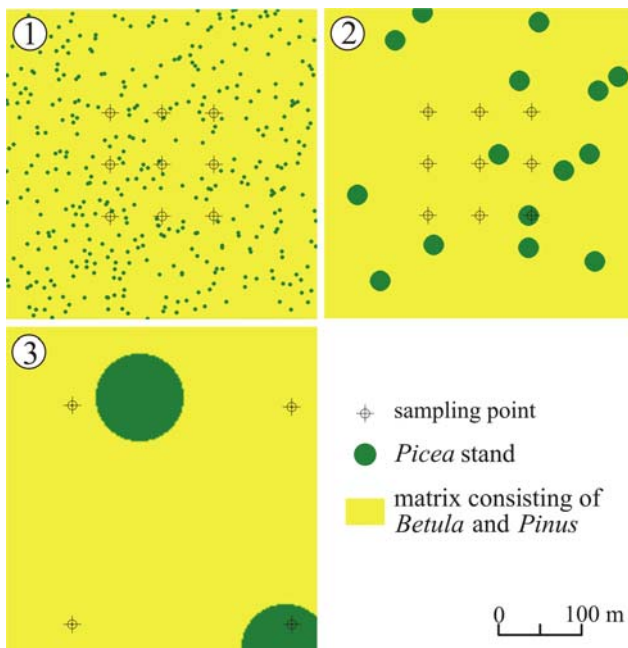
Fig. 8 Examples of random landscapes used in the three scenarios of example no. 4. Note that only a small proportion of the landscape is shown. Erratum: in scenario 3, the sampling points should be identical as in scenarios 1 and 2. Radius of Picea patches: 1. 5 m, 2. 25 m, and 3. 100 m
