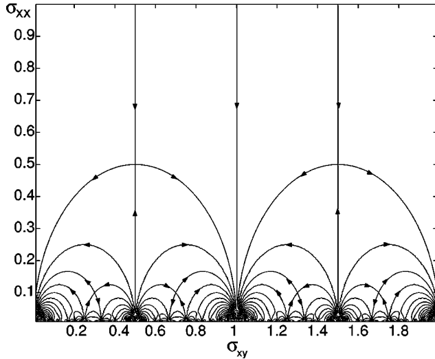
FIG. 1. Crossover flow of the conductivities as predicted from the law of corresponding states.
