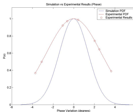
Figure 7: The Phase Simulation Results vs. Phase Experimental Results for the Top Left Reference Calibration Algorithm for a 2 by 4 array.
