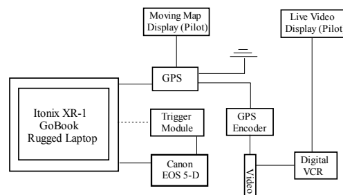
Figure 1. Schematic of data acquisition system
