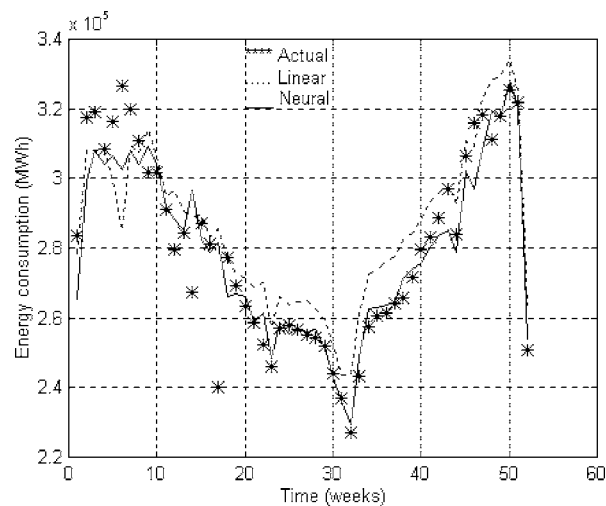
Figure 8. Forecasts using Box–Jenkins models.
