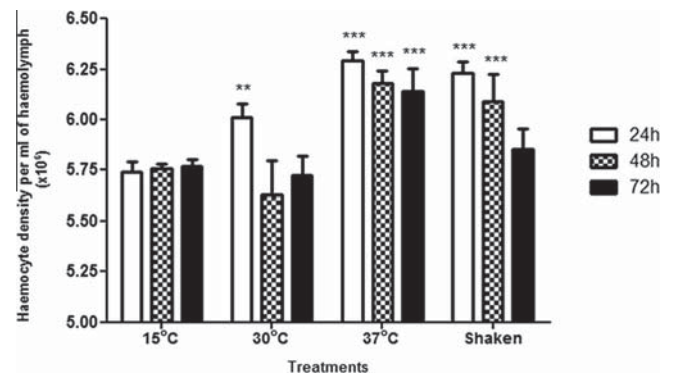
Fig. 2. Haemocyte density of larvae thermally (15 °C, 30 °C and 37 °C) or physically stressed (shaken) at 24, 48 or 72 h.
