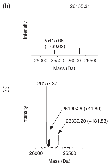
Figure 7 N-terminal sequencing and electrospray ionization quadrupole time-of-flight mass spectrometry (ESI-QTOF-MS) of purified p24. (a) N-terminal sequence of ammonium sulphate-enriched p24 from pZSJH1p24 plants and purified pZF5 chloroplast p24 pH 6.5 fraction. (b) Mass spectrum of purified pZF5 chloroplast p24 pH 6.5 fraction showing a major peak at 26 155.31 Da. The theoretical mass of a 237-amino-acid pZF5-expressed p24 protein with an N-terminus of ASGSPIVQ is 26 158 Da. The minor peak at 25 415.618 Da corresponds to the loss of eight amino acid residues (ASGSPIVQ, 739.83 Da) from the pZF5 p24 N-terminus. (c) Mass spectrum of purified pZF5 chloroplast p24 pH 6.2, 6.7, 6.9, 7.2 fractions combined showing the major peak at 26 157.37 Da. Masses indicated are labels that were added to the peaks by the software linked to the QTOF instrument. For additional peaks, masses relative to the major peak are indicated in brackets.
