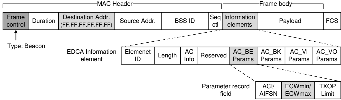
Figure 3: Structure of a beacon management frame. Fields modified to generate unicast beacons that configure individual clients are highlighted. The destination address field is changed from broadcast to that of the target station. ECWmin and ECWmax settings are updated with the values that solve utility maximisation.
