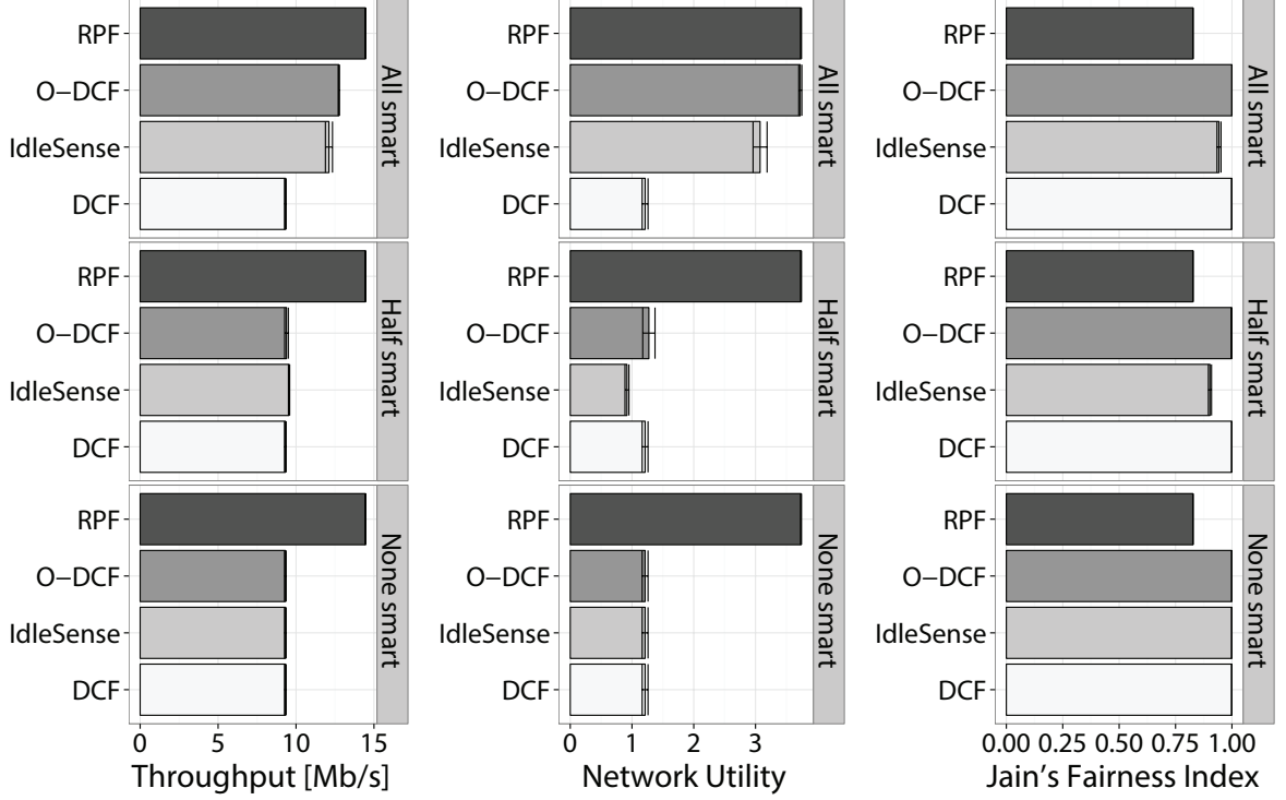
Figure 11: WLAN with 8 backlogged stations transmitting using UDP. Stations use the OFDM PHY layer (802.11a), fully heterogeneous bit rates and employ our proposal (RPF), Idle Sense, O-DCF, and standard DCF. Total throughput (left), network utility (centre), and Jain's fairness index (right) in three scenarios: all clients smart (implementing changes as required, top), half smart (middle), and respectively all legacy (none smart, bottom). Simulations results.
