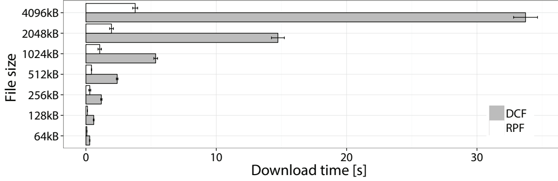
Figure 8: WLAN with 2 stations: one downloads small-sized files from the AP using HTTP over a link operating at 54Mb/s; the other is backlogged and uploads to the AP using TCP over a 6Mb/s link. Download time of different-size objects with DCF and the proposed RPF scheme. Experimental data.
