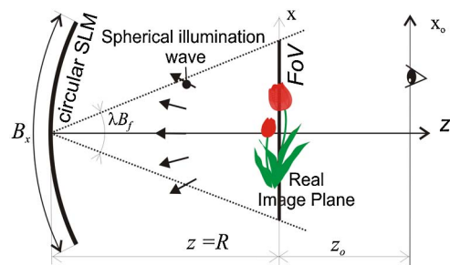
Fig. 1. (Color online) Holographic display system with theoretical circular SLM.
