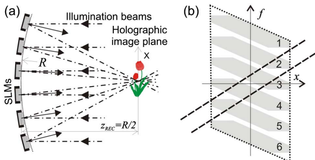
Fig. 3. (Color online) (a) Illustration of the holographic display system with planar SLMs aligned on a circle. (b) WDF representation of the optical signal generated at plane z = R in a display, the dotted line illustrates the WDF of the circular display and the gray regions illustrate the WDF of the display built from planar SLMs. The larger dashed line illustrates the WDF of an eye aperture that is backpropagated to the image plane.
