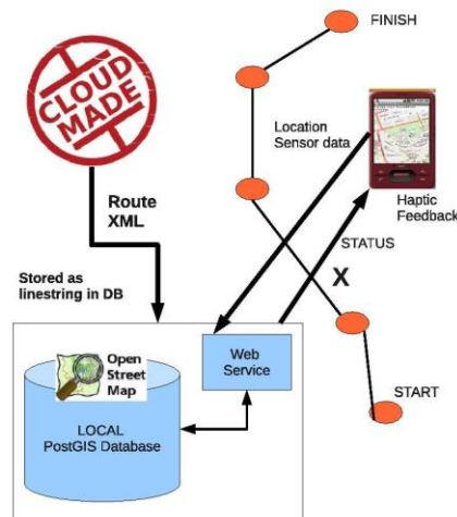
Figure 1: A schematic of the components in our pedestrian navigation application
