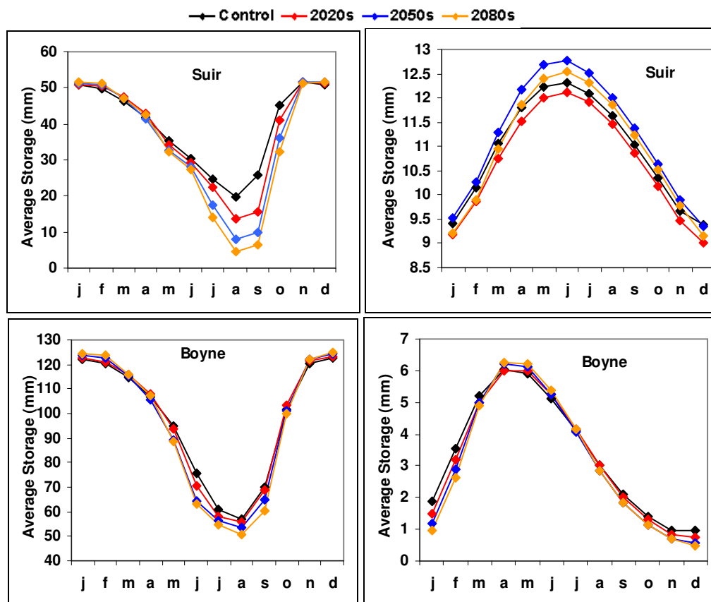
Figure 1 Changes in catchment storage simulated for the Suir and the Boyne catchments using the mean ensemble.
