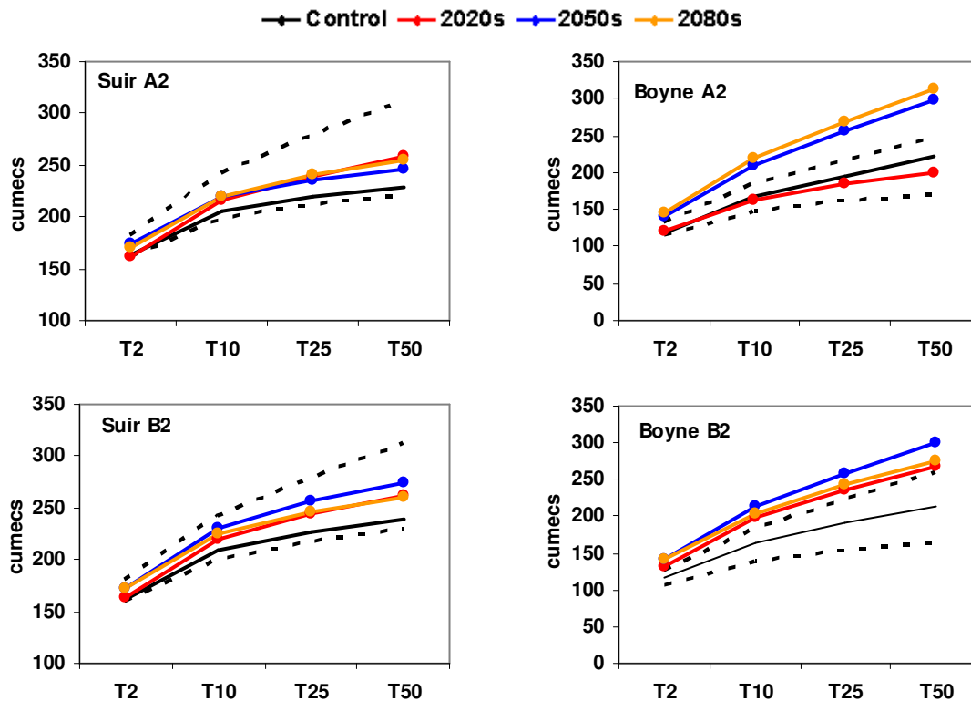
Figure 3 Changes in the magnitude of selected flood events in the Suir and the Boyne under the A2 and B2 emission scenarios. Changes are represented as the average change simulated by each GCM.
