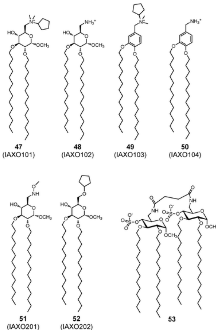
Fig. 17 Synthetic lipids with TLR4-modulating activity.
