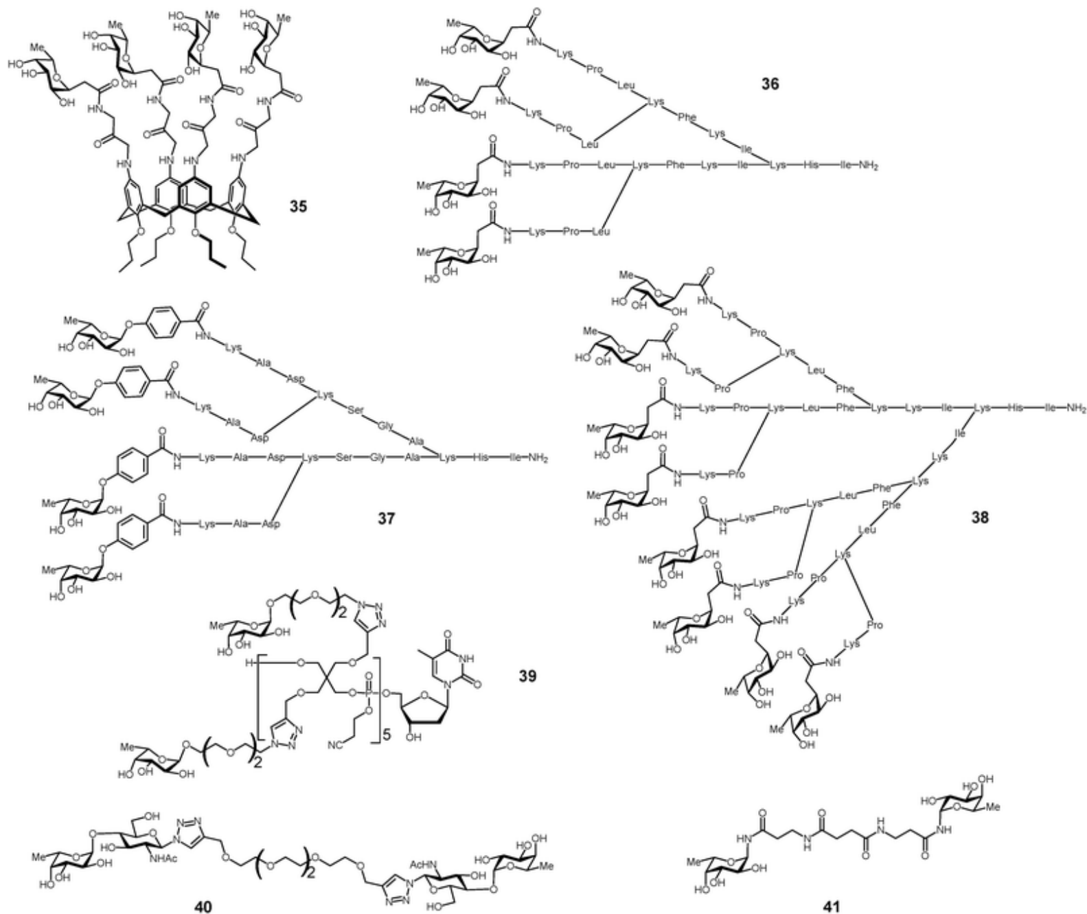
Fig. 11 Multivalent glycoconjugates 35–41 as LecB high affinity ligands.
