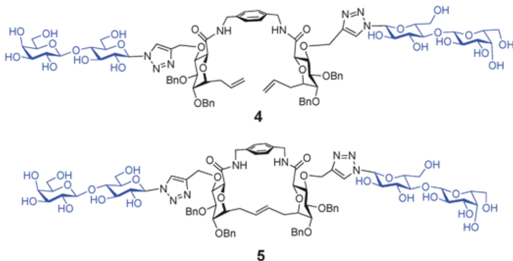
Fig. 3 Bivalent glycoclusters 4 (acyclic) and 5 (macrocyclic), identified as sensors for different galectin subtypes.
