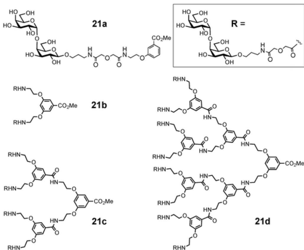
Fig. 8 Oligovalent galabiose derivatives.
