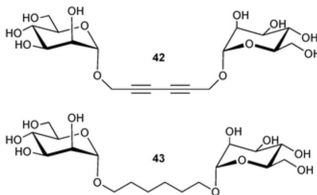
Fig. 12 Divalent mannose ligands as ligands of BC2L.
