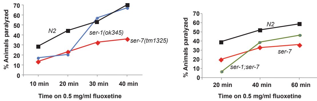
FIGURE S2.—The time course of fluoxetine-induced paralysis. The assay has been performed multiple times, and the data from one experiment are presented.
