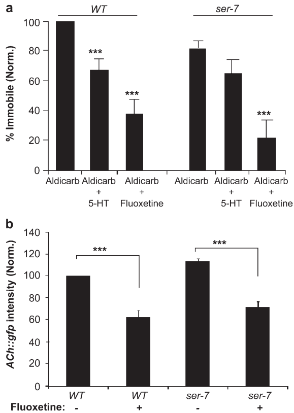
FIGURE 5.—Action of fluoxetine and 5-HT on ACh in ser-7 mutants. (a) Aldicarb-induced immobility of animals pretreated with 5-HT (5 mg/ml) or fluoxetine (0.5 mg/ml) or without pretreatment. The values of the mutants and pretreated animals are normalized to that of WT animals without pretreatment. (b) Fluoxetine downregulates ACh::gfp in WT and ser-7 mutant animals. Intensity of the fluorescence in the 9th and 10th neurons from the anterior (as shown in Figure 3b) was quantified. The values of WT animals treated with fluoxetine (0.5 mg/ml, 24 hr) and the ser-7(tm1325) mutant untreated and treated with fluoxetine are normalized to that of untreated WT assayed on the same day. Each bar represents at least three replicate experiments \pm SEM. *** P < 0.001 , Student's t -test.
