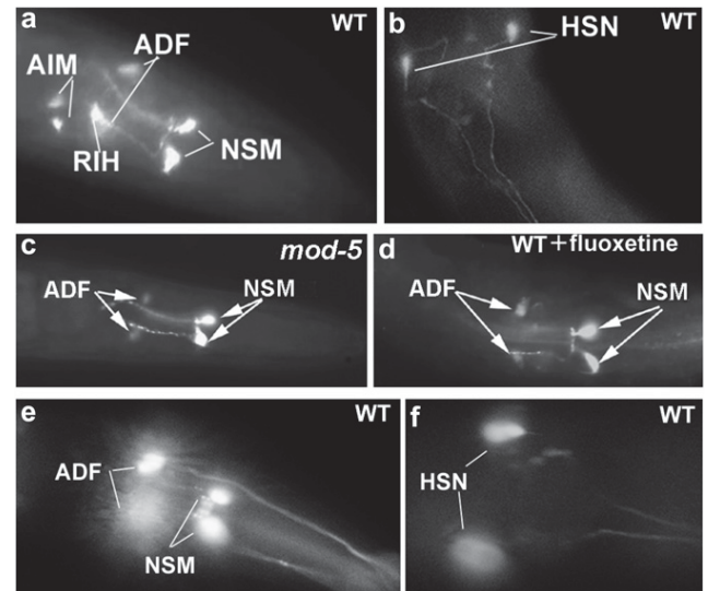
FIGURE 1.—Fluoxetine treatment and mutations in mod-5 /SERT abolish anti-5-HT immunoreactivity in the RIH and AIM neurons. (a–d) Photomicrographs of animals stained with anti-5-HT antibodies. To test the effects of MOD-5/SERT inhibitors, WT animals were incubated overnight on NGM plates containing 0.5 mg/ml of fluoxetine (as shown) or 0.4 mg/ml of imipramine (not shown) before fixation for staining. (e and f) Photomicrographs of WT animals expressing tph-1::gfp . All the animals shown have anterior to the right.
