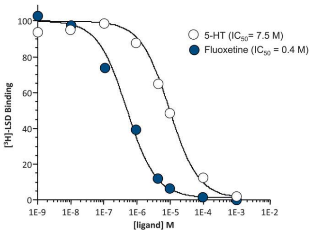
FIGURE 8.—Fluoxetine binds to SER-7. The membrane fraction of COS-7 cells transiently expressing the SER-7b isoform was incubated with 10 nM [ ^3 H]LSD alone or in the presence of 5-HT or fluoxetine at the indicated concentrations. The data are representative of at least three experiments, each performed in triplicate. Each point is the mean \pm SEM.
