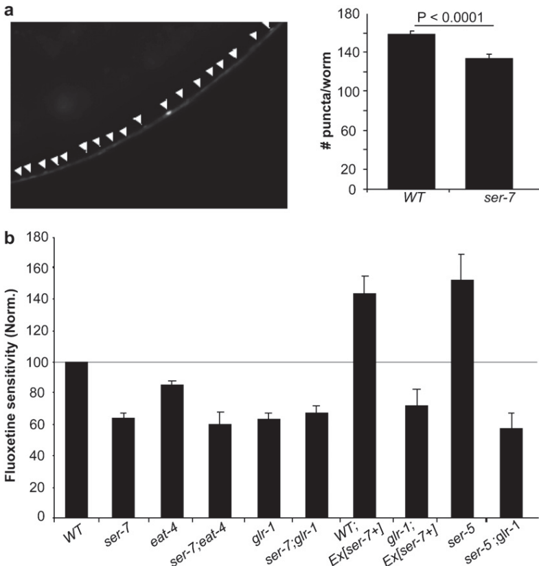
FIGURE 7.—Genetic interaction between glr-1 , ser-5 , and ser-7 . (a) Quantification of GLR-1::GFP puncta in WT and ser-7(tm1325) animals. GLR-1::GFP is localized to the punctate structure along the ventral nerve cord (RONGO et al. 1998). Individual GLR-1::GFP puncta in 1-day-old adults, genotype blinded, were counted under a fluorescence microscope, N = 15 per strain. The P -value is indicated on the top of the bar (Student's t -test). (b) Fluoxetine-induced paralysis. The percentage of paralyzed animals, normalized to that of WT assayed on the same day, is shown for the mutants and transgenic animals. Each bar represents three replicate experiments \pm SEM. The differences between glr-1 and ser-5; glr-1 and the differences between glr-1; ser-7; glr-1 , and glr-1; Ex[ser-7(+)] are not significant ( P > 0.1 , Student's t -test).
