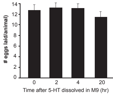
FIGURE S4.—Analysis of 5-HT stability in solution. The stability of 5-HT in solution was evaluated by testing its ability to induce egg laying in WT animals. 5-HT was dissolved in M9 buffer to give the final concentration of 5 mg/ml 5HT, and the solution was stored in dark at 20°C. To test the response to 5-HT, animals were placed individually into wells of a 96-well plate, with each containing 100 ml of M9 buffer or M9 buffer containing 5-HT. The number of eggs laid was scored after 60 min. Animals did not laid egg in M9 buffer (data not shown) (Trent et al. 1983). There is no significant difference in the number of eggs laid between animals incubated in the solution at these four time points ( p > 0.4 Student's t-test).
