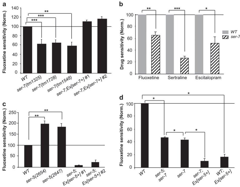
FIGURE 4.—SSRI-induced paralysis in ser-5 and ser-7 mutants. Larval stage four (L4) worms were incubated for 24 hr in liquid media supplemented with a drug: 0.5 mg/ml fluoxetine (a and d); 0.5 mg/ml fluoxetine, 0.25 mg/ml sertraline, and 2.25 mg/ml escitalopram (b); and 0.25 mg/ml fluoxetine (c). Drug sensitivities were calculated as described in Figure 2d. The values of the mutants are normalized to that of WT assayed in parallel. Two transgenic lines each for Ex[ser-7(+)] and Ex[ser-5(+)] were assayed. Each bar represents at least three independent experiments \pm SEM. * P < 0.05 , ** P < 0.01 , *** P < 0.001 , Student's t -test.
