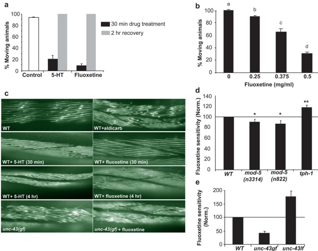
FIGURE 2.—Fluoxetine and 5-HT cause muscle relaxation. (a) The percentage of WT worms moving in M9 (open bar) and in M9 supplemented with 5 mg/ml 5-HT or 0.5 mg/ml fluoxetine (solid bars). The paralyzed animals resumed locomotion after they were transferred to standard culture plates (shaded bars). Each bar represents the mean of three independent experiments, each performed with three replicates \pm SEM. One-day-old adults were tested. (b) Dosage dependence of the paralytic effect of fluoxetine in WT animals. Larval stage four (L4) worms were incubated for 24 hr in liquid media without fluoxetine or containing fluoxetine at indicated concentrations. Each bar represents the mean of three independent experiments, each performed with three replicates \pm SEM. Different letters represent a significant difference (one-way ANOVA, P < 0.05 ). (c) Visualization of body-wall muscle sarcomeres in living C. elegans . WT animals expressing an integrated MYO-3::GFP transgene were incubated for 30 min or 4 hr in media without drug or supplemented with 5 mg/ml 5-HT, 0.5 mg/ml fluoxetine, or 0.8 mM aldicarb. One-day-old adults were examined. (d and e) Quantification of fluoxetine-induced paralysis in WT and mutants. Fluoxetine sensitivity was scored by calculating the percentage of worms paralyzed following 24-hr incubation in liquid media supplemented with 0.5 mg/ml fluoxetine. The values of each mutant strain are normalized to that of WT worms assayed in parallel. Each bar represents the mean of three independent experiments \pm SEM. * P < 0.05 , ** P < 0.01 , Student's t -test. In a and c, the assays were performed with animals in culture media without food, allowing fast ingestion of the drugs, and thus likely reflecting the maximal speed of drug effects. In b, d, e, and all other experiments described in this article the assays were performed with well-fed animals, reflecting optimal physiological conditions.
