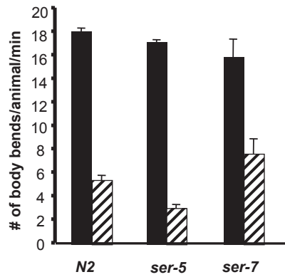
FIGURE S3.—Effects of 5-HT treatment on locomotion in WT, ser-5 and ser-7 mutant animals. One-day old animals were transferred onto NGM plates supplemented with 5 mg/ml 5HT (hatched bars) or without 5-HT (black bars) for 15 min. The number of body bends of individual animals was scored by continuously monitoring individual animals for 20 seconds. In the presence of 5-HT, locomotion of ser-5 mutants was slower than that of WT ( p < 0.05 ). However, the difference between WT and the ser-7 mutant animals is not significant ( p > 0.05 ). Student's t-test.
