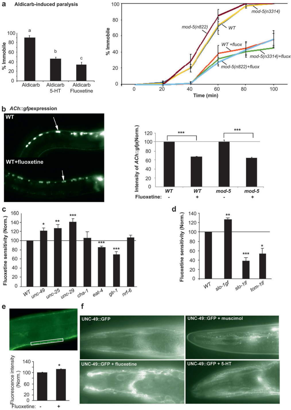
FIGURE 3. —Action of fluoxetine and 5-HT on the ACh, GABA, and glutamate systems. (a) Aldicarb-induced paralysis of animals pretreated with 5-HT or fluoxetine and without pretreatment. Left, the percentage of worms paralyzed after 60 min of exposure to aldicarb. Right, the time course of aldicarb-induced paralysis. The error bars indicate SEM ( n > 3 replicates). Different letters represent a significance difference (one-way ANOVA, P < 0.05 ). (b) Fluoxetine downregulates ACh::gfp in WT and mod-5 mutant animals. Left, photomicrographs of ACh::gfp expression in animals untreated and treated with fluoxetine (0.5 mg/ml, 24 hr). Right, intensity of ACh::gfp in L4 animals without and with fluoxetine treatment was quantified by measuring the fluorescence in 9th and 10th neurons from the anterior (indicated in the photomicrographs by arrows) in individual animals. Each bar represents three independent experiments \pm SEM. *** P < 0.001 , Student's t -test. (c and d) Fluoxetine sensitivity of ACh, GABA, and glutamate mutants. Fluoxetine sensitivities were measured as described in Figure 2d. Each bar represents three independent experiments \pm SEM. * P < 0.05 , ** P < 0.01 , *** P < 0.001 , compared to WT, Student's t -test. (e and f) UNC-49::GFP expression in WT animals treated with 5-HT and fluoxetine. (e) Quantification of the fluorescence within an area of 50 \times 5 \mu\text{m} at the loco-
