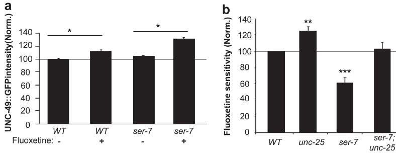
fluoxetine. * P < 0.05 , Student's t -test. (b) Fluoxetine-induced paralysis. Fluoxetine sensitivity was calculated as described in Figure 2d. Each bar represents three replicate experiments \pm SEM. ** P < 0.01 , *** P < 0.001 . There is no significant difference between WT and ser-7; unc-25 ( P > 0.9 , Student's t -tests).
