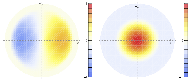
FIG. 4: (Color online) False color plot of magnetization integrated in-situ, symmetry broken the along z -axis. Hedgehog imaged along the x -axis (left) and skyrmion imaged along the z -axis (right).
