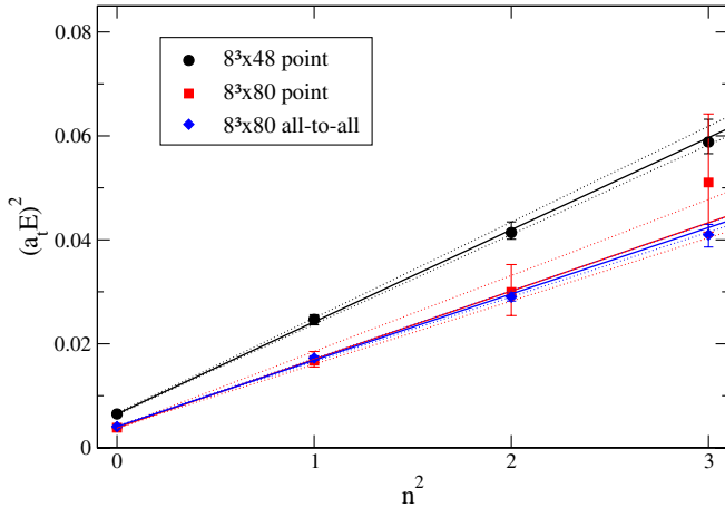
FIG. 2 (color online). A comparison of the dispersion relations determined from an 8^3 \times 48 lattice and an 8^3 \times 80 lattice. The solid lines are the best fits and the dotted lines are the 68% confidence levels. The figure also shows a comparison of all-to-all propagators and point propagators on the same (longer) lattice. The plot shows that the ground state energies have not reached a plateau on the shorter lattice. On the longer lattice the all-to-all and point data agree, while higher precision is achieved with all-to-all propagators.
