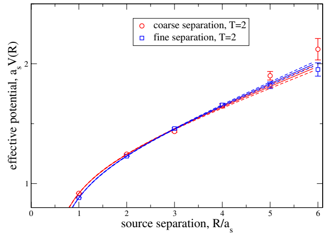
FIG. 6 (color online). The potential between fundamental static color sources for run 6, measured from static propagation in a coarse direction. Lines show fits to the Cornell potential, and are used in a crude determination of the lattice spacing.
