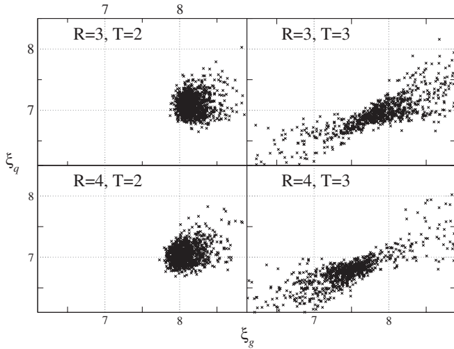
FIG. 4. Tuned values of input parameters ( \xi_g^0 , \xi_q^0 ) determined from the plane fit procedure on the 8^3 \times 80 lattice. The plots show the results for different values of R and T used to determine the gluon anisotropy. Each point corresponds to one bootstrap sample.
