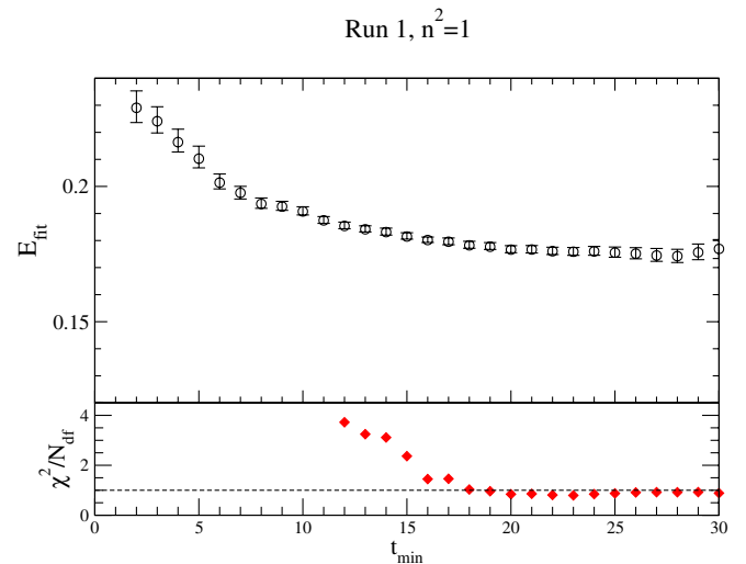
FIG. 1 (color online). A typical t_{\min} plot, showing the energy for momentum n^2 = 1 on run 1, 8^3 \times 80 lattices from fits to time ranges t_{\max} = 40 for various t_{\min} . A stable ground state energy determination, with a good \chi^2 , is achieved for 22 \leq t_{\min} \leq 30 .
