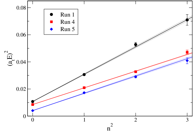
FIG. 3 (color online). Dispersion relations from runs 1, 4 and 5 on 8^3 \times 80 lattices using all-to-all propagators. The solid line is a fit to the four points and the dotted lines are the 68% confidence levels. The quality of all three fits is very good with \chi^2/N_{\text{d.f.}} = 2.0/2, 1.9/2, 2.0/2 for runs 1, 4 and 5, respectively.
