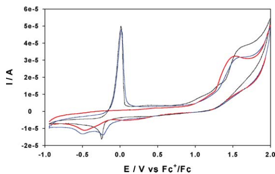
Fig. 8 Cyclic voltammograms describing the electrochemical behaviour of 1:1 solution mixtures of \text{AgClO}_4 - 3 , cycle 1 (solid black trace) and \text{AgClO}_4 - 3 , cycle 10 (solid blue trace). The solid red trace is 1 \times 10^{-3} M 3 only. All data recorded in 0.1 M TBAPF 6 in MeCN at a scan rate of 100 mV s -1 .
