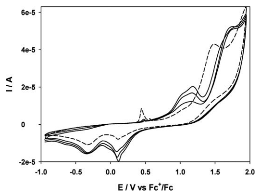
Fig. 7 The effect of \text{Hg}(\text{ClO}_4)_2 on the oxidation of 3 in MeCN and 0.1 M TBAPF 6 . The scan rate employed was 100 mV s -1 .
