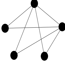
Fig. 1. Graph with 5 vertices, k = 2 and q_1(G) = 6.3722 > 2n - 4
