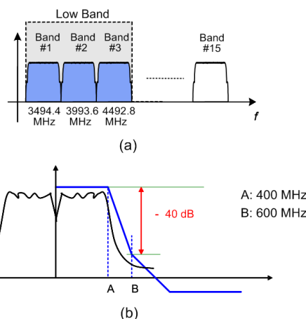
Figure 1. Impulse UWB channel selection requirement for LPF
