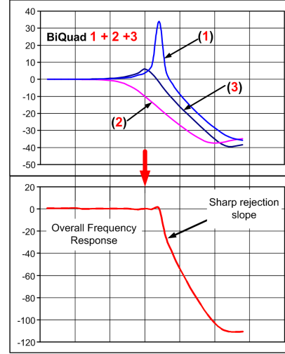
Figure 3. Three different AC characteristic of the three Biquads.
