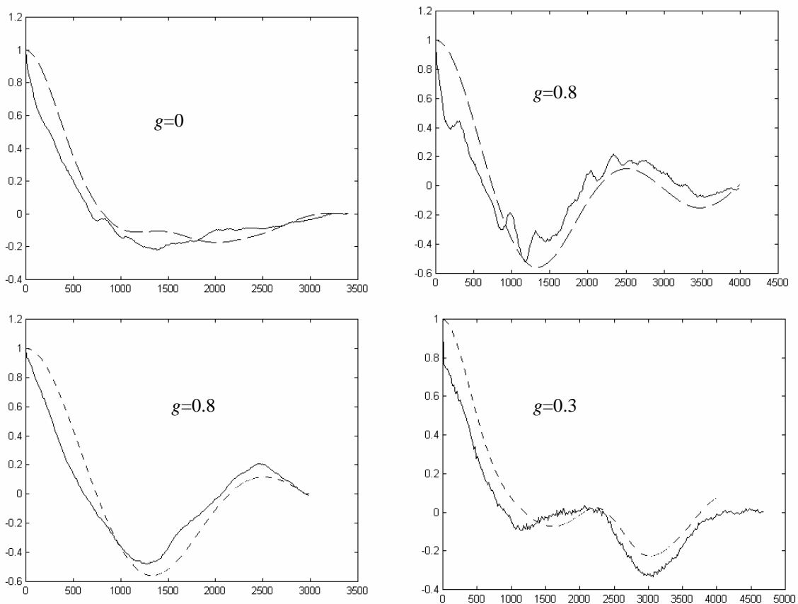
Figure 5 Subject (solid line) and model (dashed line) autocorrelograms. Abscissae are in milliseconds and ordinates normalised.
